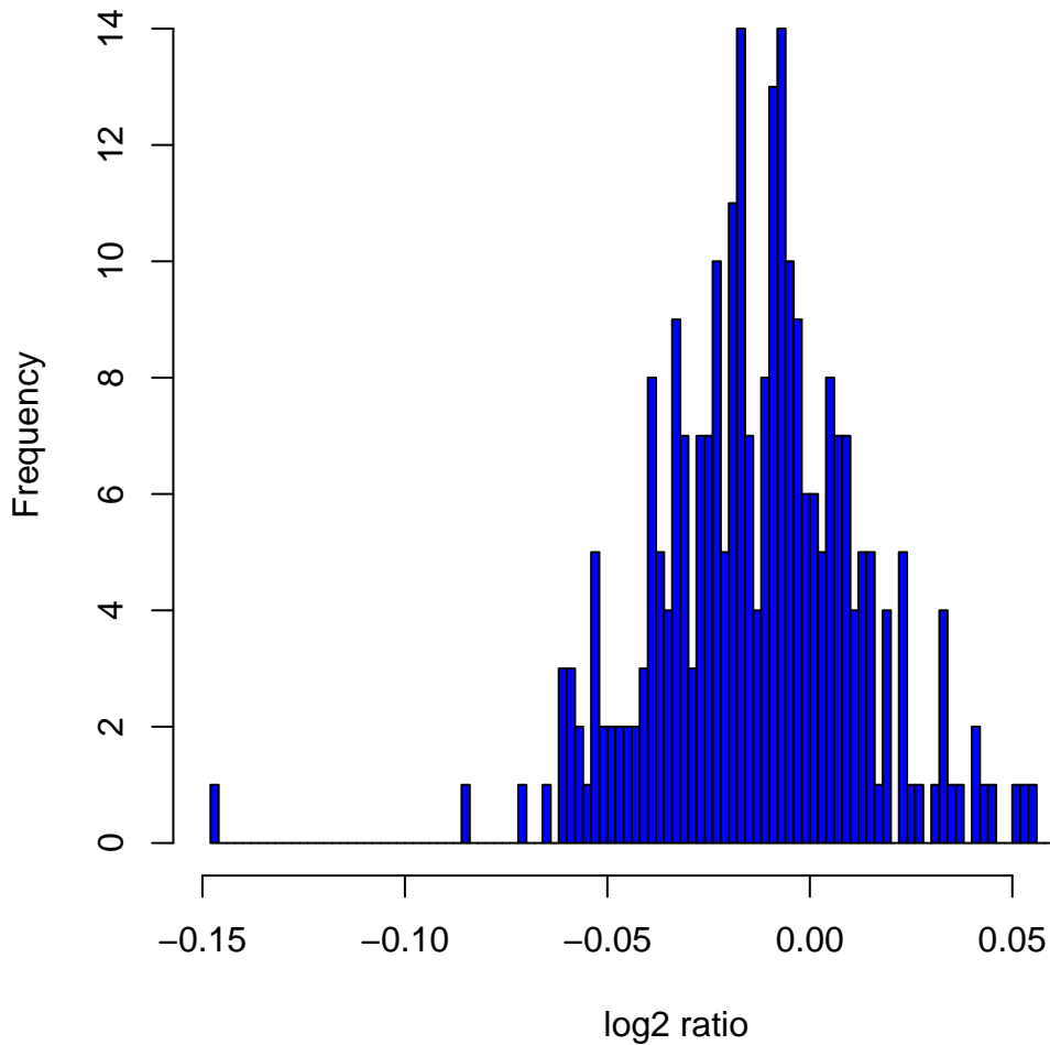
Histogram of log2ratios in 270 HapMap samples at clone Chr5tp-20C12
