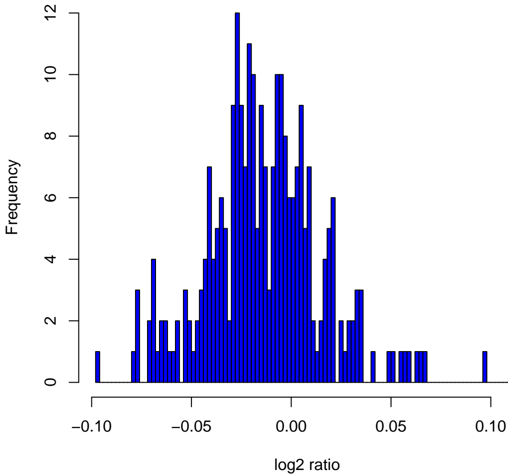
Histogram of log 2 ratios in 270 HapMap samples at clone Chr5tp-20C2
