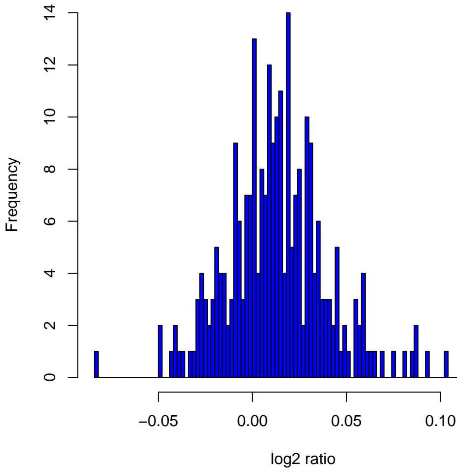
Histogram of \log_2 ratios in 270 HapMap samples at clone Chr5tp-20D2
