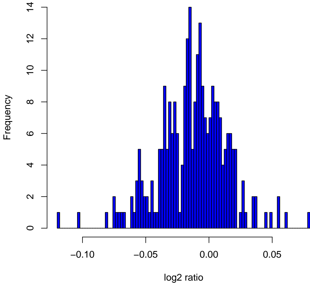
Histogram of log 2 ratios in 270 HapMap samples at clone Chr5tp-20G3
