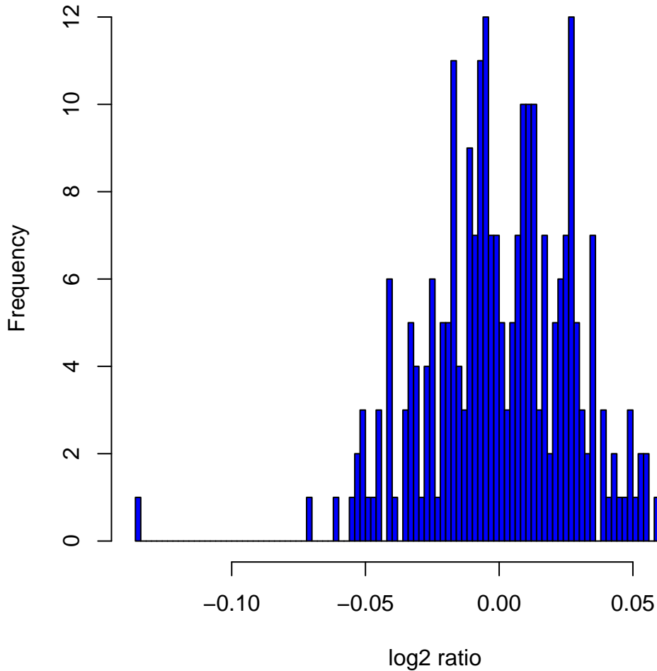
Histogram of log 2 ratios in 270 HapMap samples at clone Chr5tp-20H4
