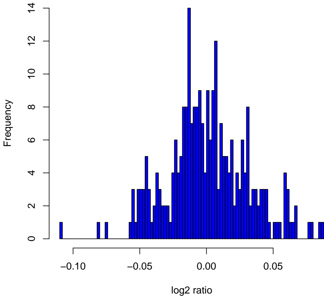
Histogram of log 2 ratios in 270 HapMap samples at clone Chr5tp-20H8
