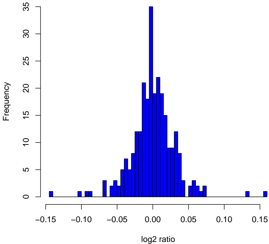
Histogram of \log_2 ratios in 270 HapMap samples at clone Chr5tp-21D12
