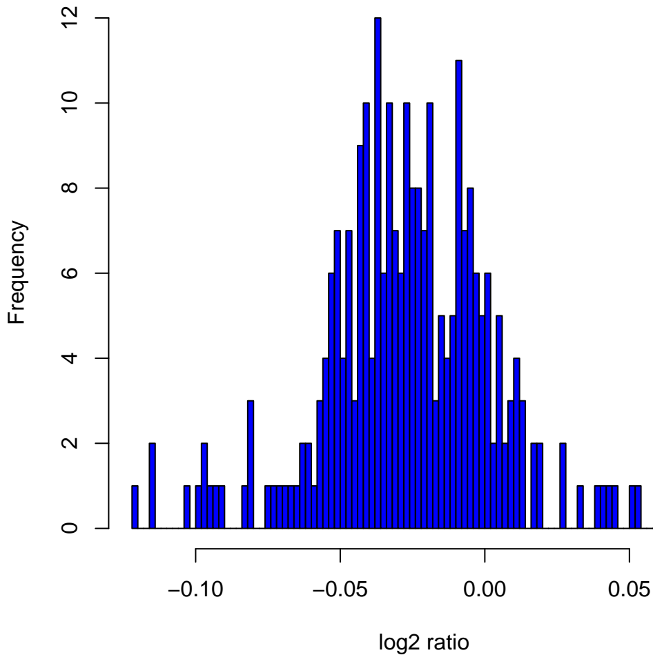
Histogram of log 2 ratios in 270 HapMap samples at clone Chr5tp-21H9
