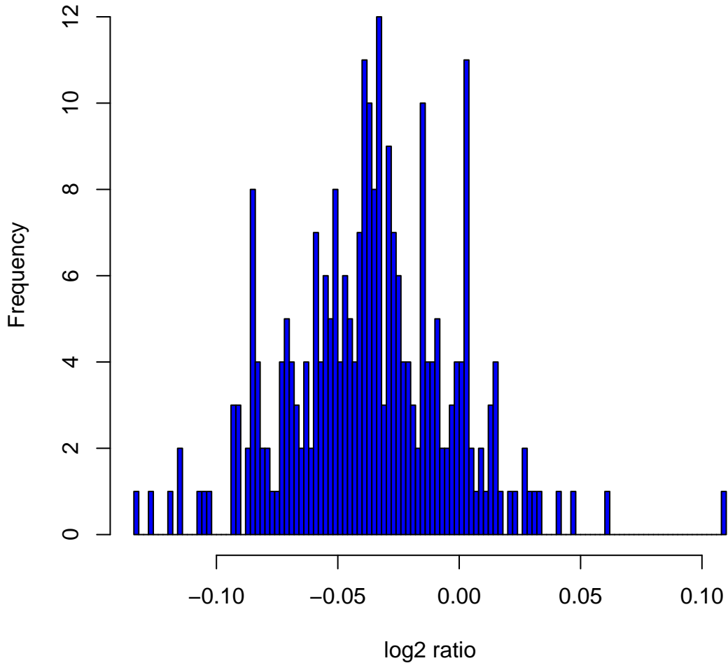
Histogram of log2ratios in 270 HapMap samples at clone Chr5tp-22A11
