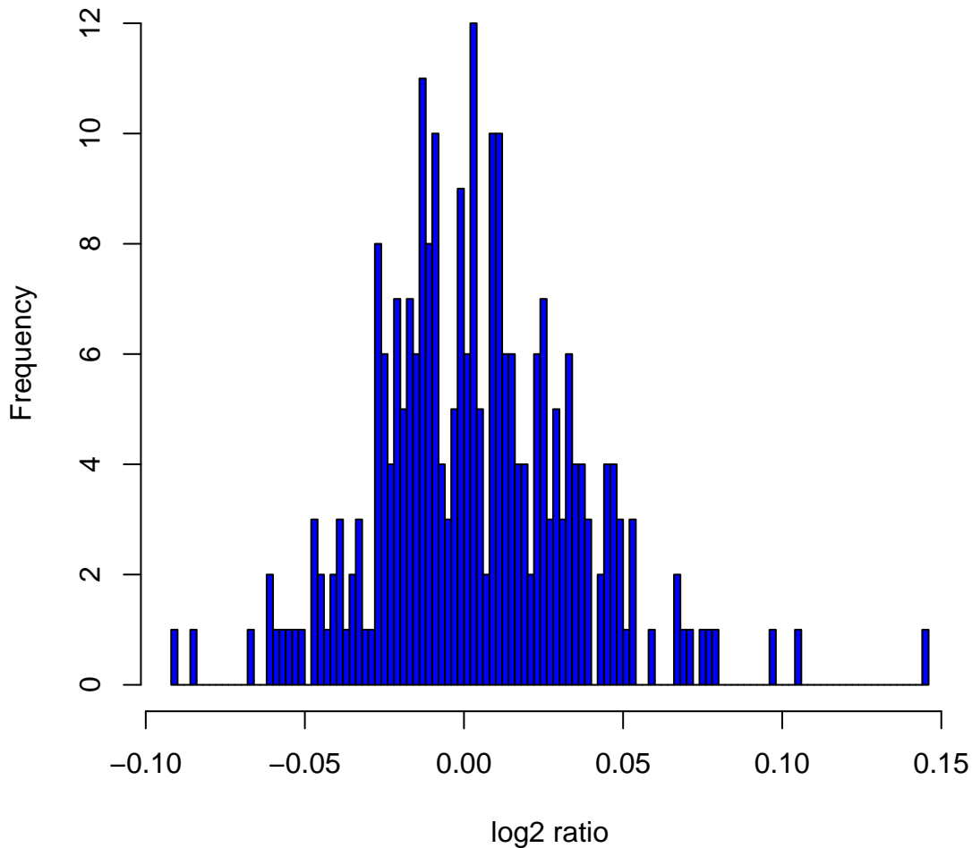
Histogram of log2ratios in 270 HapMap samples at clone Chr5tp-22B12
