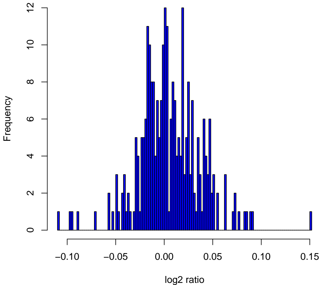
Histogram of \log_2 ratios in 270 HapMap samples at clone Chr5tp-22D8
