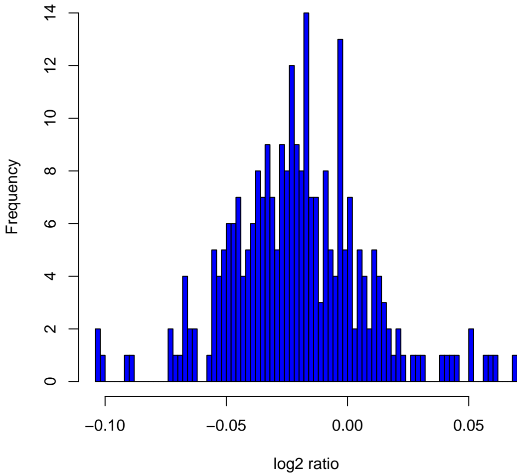
Histogram of log2ratios in 270 HapMap samples at clone Chr5tp-22F12
