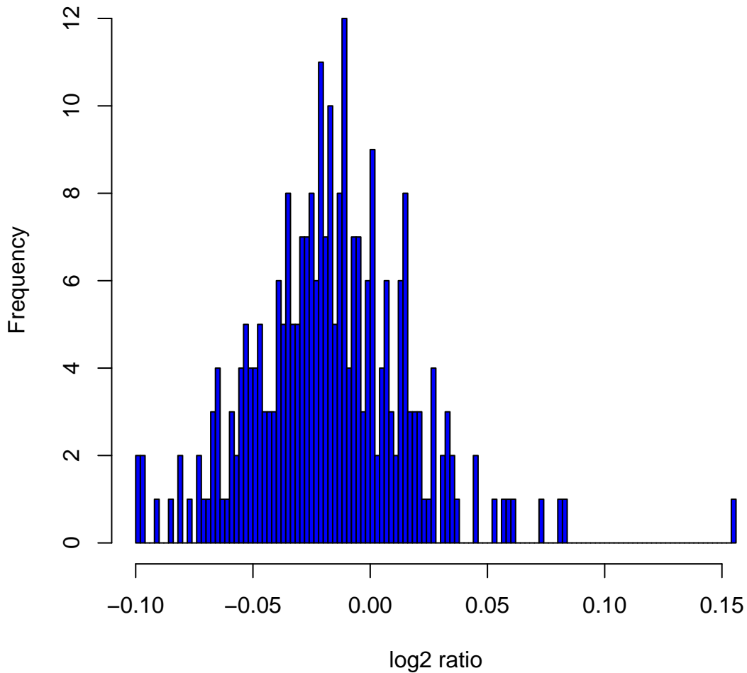
Histogram of \log_2 ratios in 270 HapMap samples at clone Chr5tp-22G10
