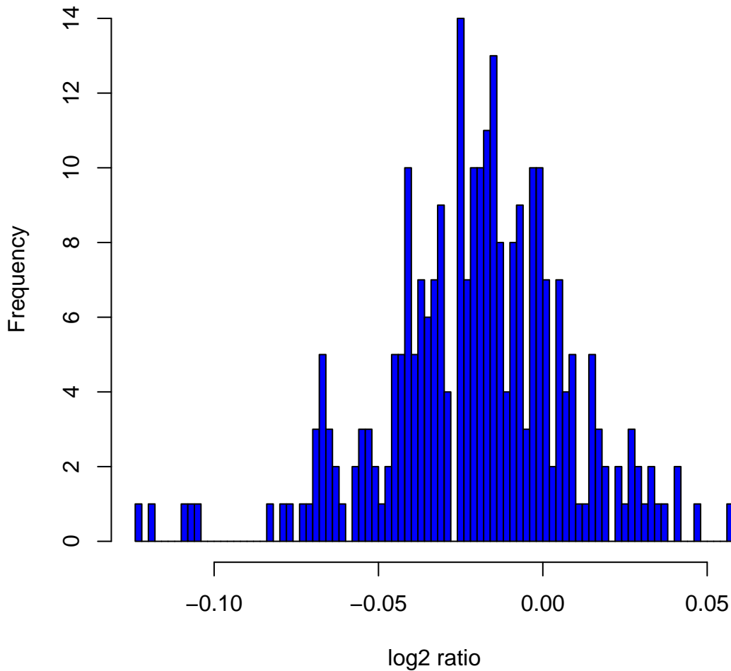
Histogram of log 2 ratios in 270 HapMap samples at clone Chr5tp-22G7
