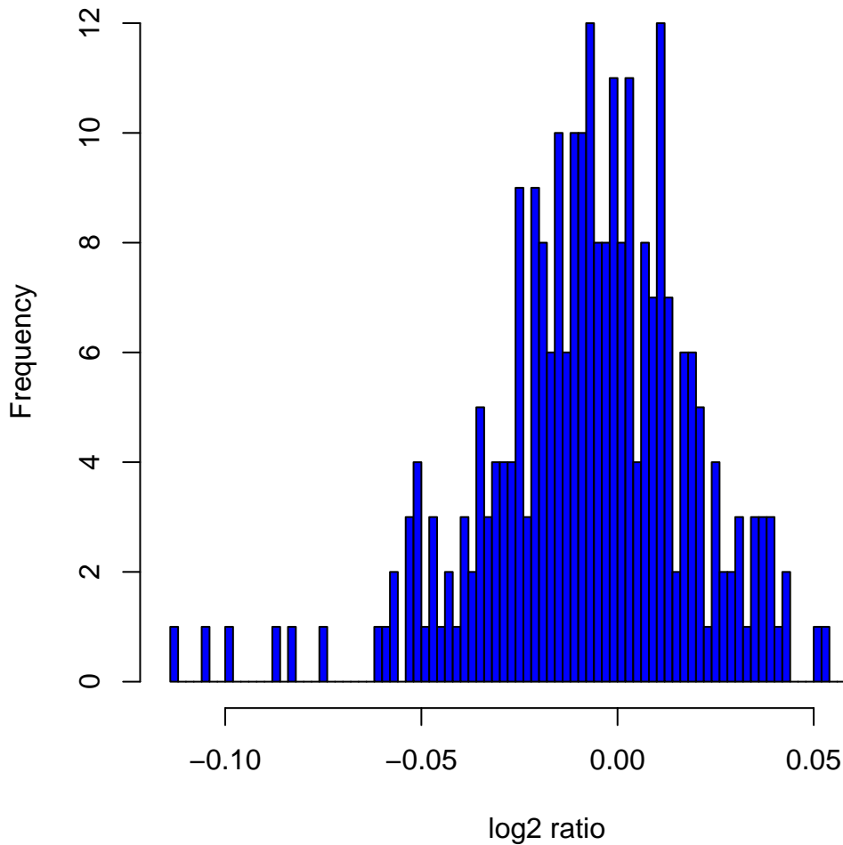
Histogram of log 2 ratios in 270 HapMap samples at clone Chr5tp-23H6
