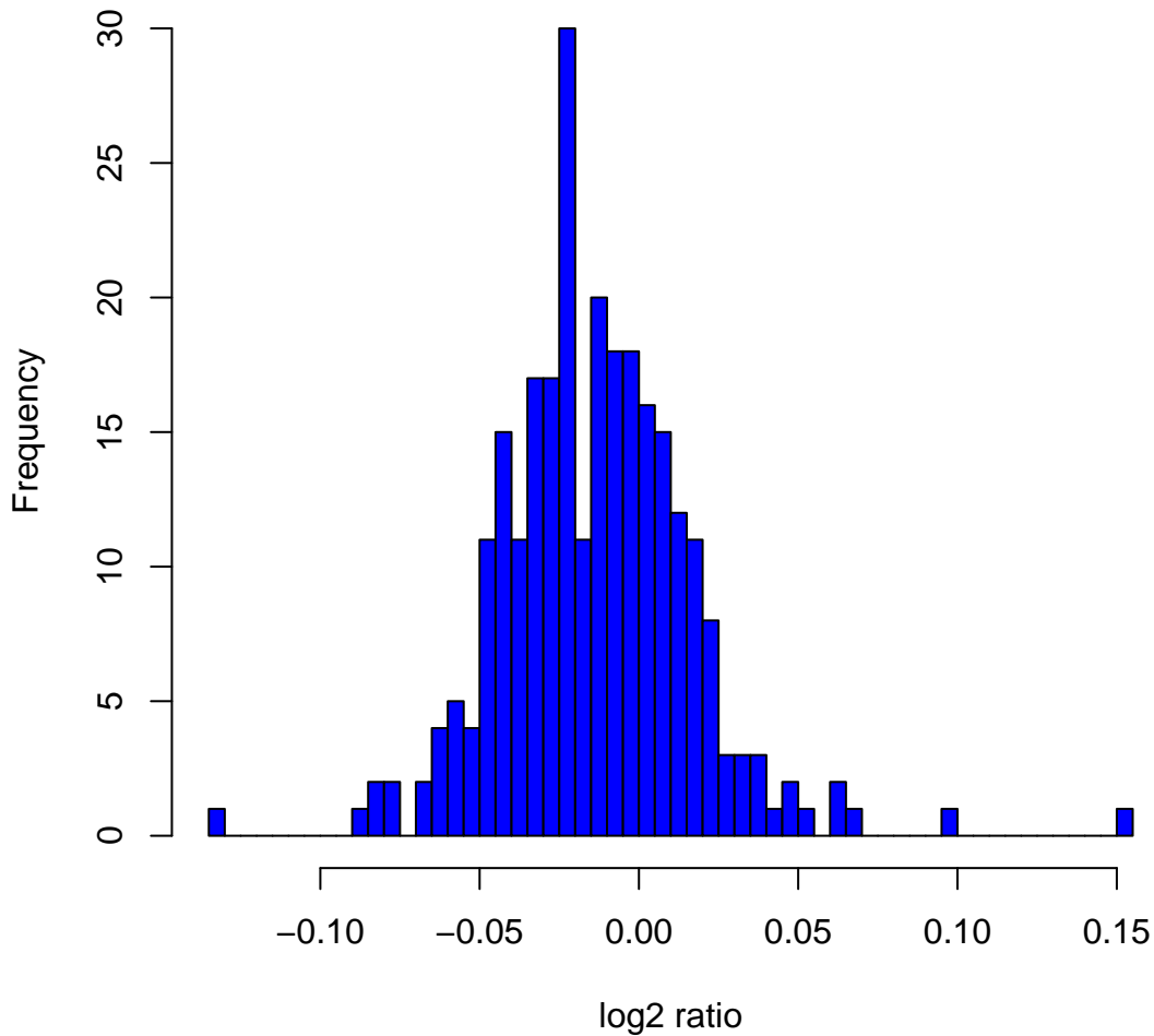
Histogram of log2ratios in 270 HapMap samples at clone Chr5tp-24B10
