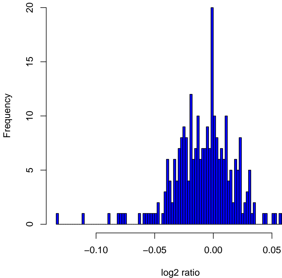
Histogram of log2ratios in 270 HapMap samples at clone Chr5tp-24E10
