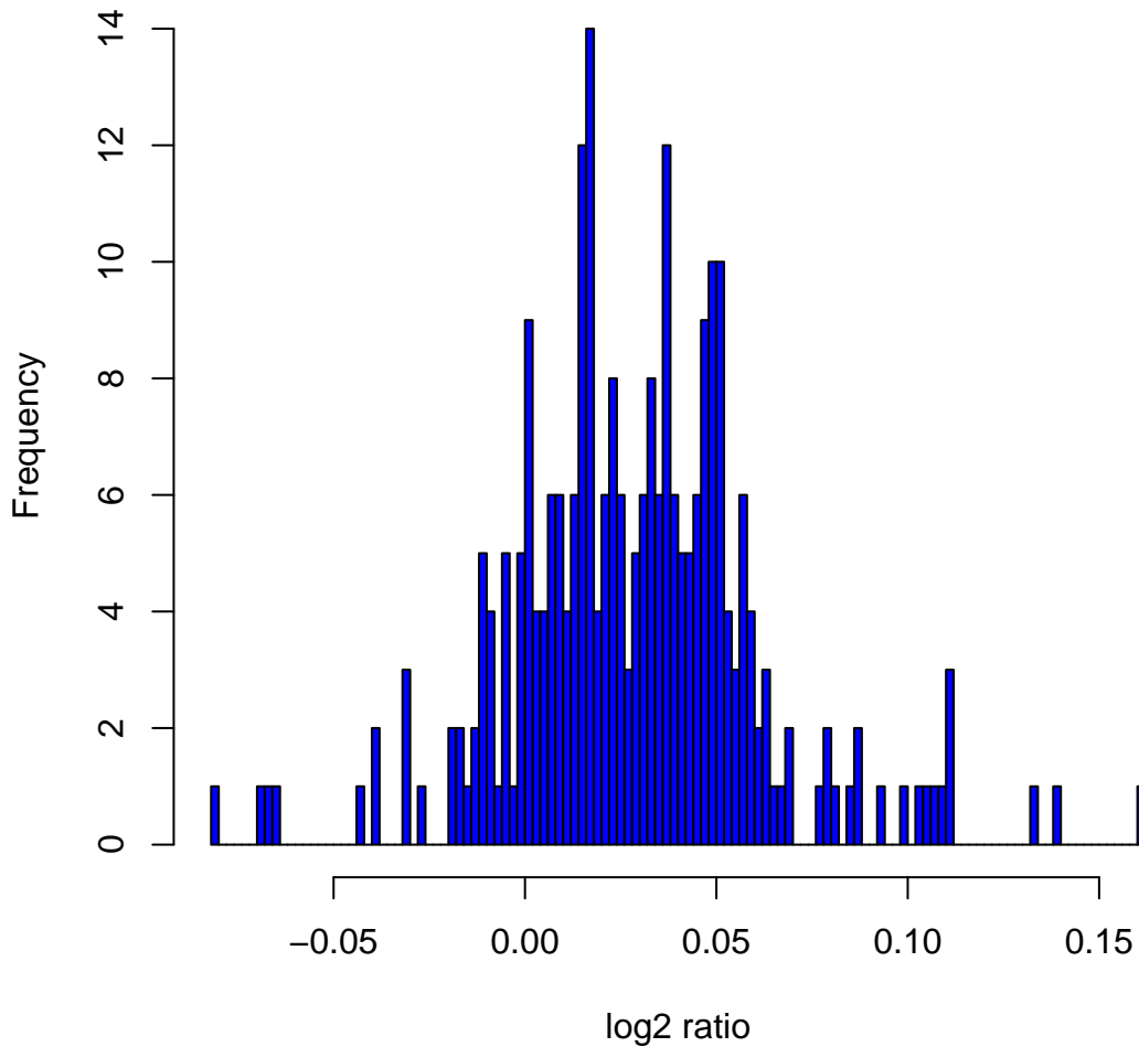
Histogram of log2ratios in 270 HapMap samples at clone Chr5tp-24F10
