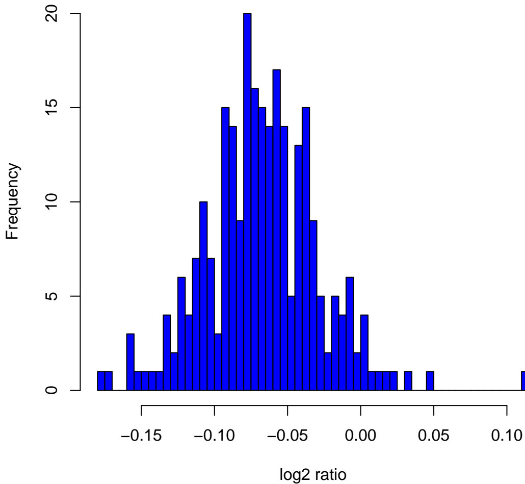
Histogram of log2ratios in 270 HapMap samples at clone Chr5tp-24H10
