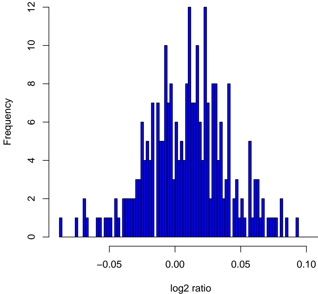
Histogram of log2ratios in 270 HapMap samples at clone Chr5tp-25A6
