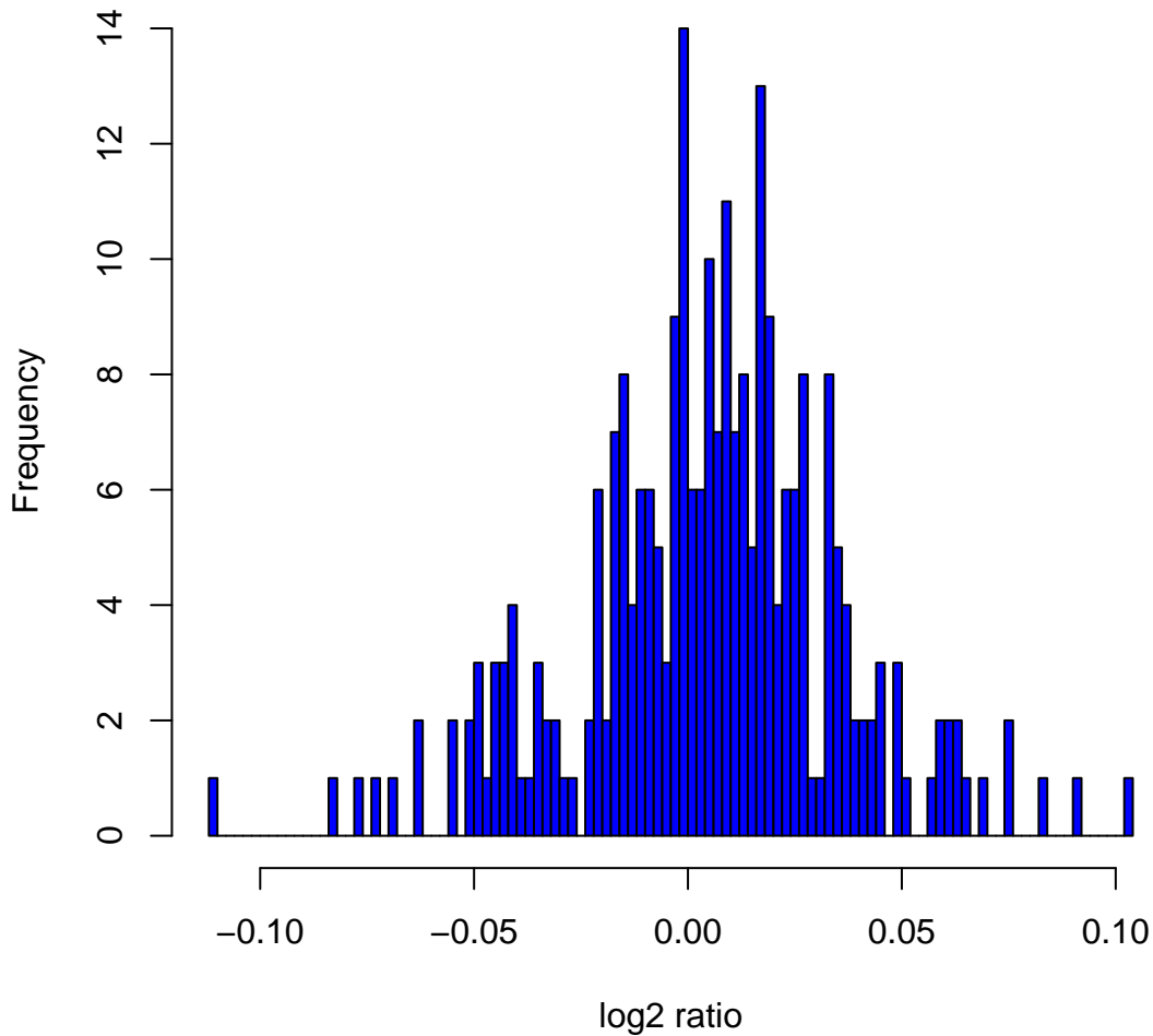
Histogram of log 2 ratios in 270 HapMap samples at clone Chr5tp-25B1
