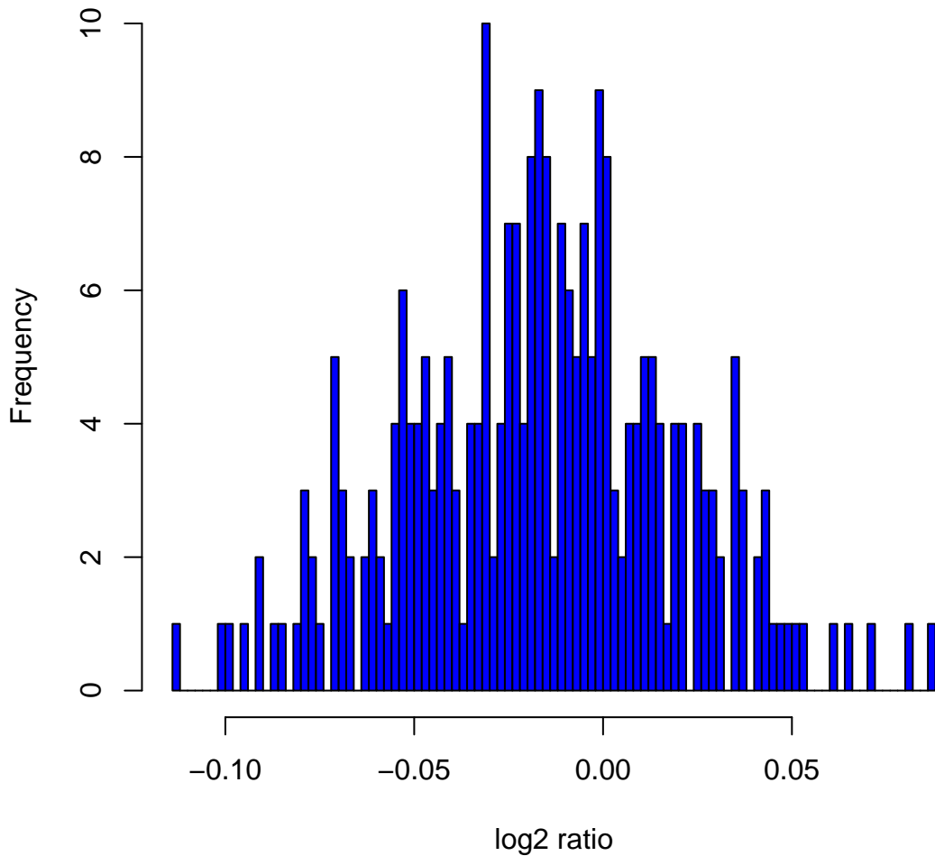
Histogram of log2ratios in 270 HapMap samples at clone Chr5tp-25D10
