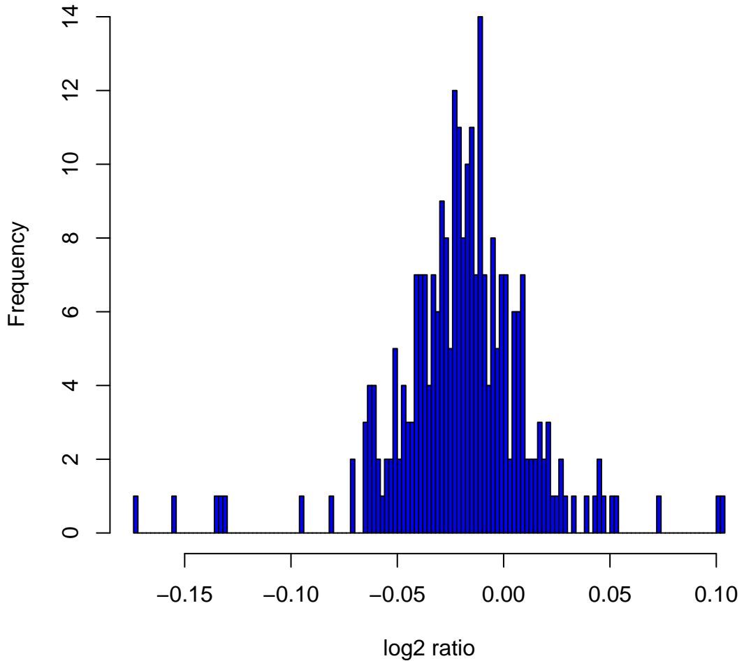
Histogram of log2ratios in 270 HapMap samples at clone Chr5tp-25E11
