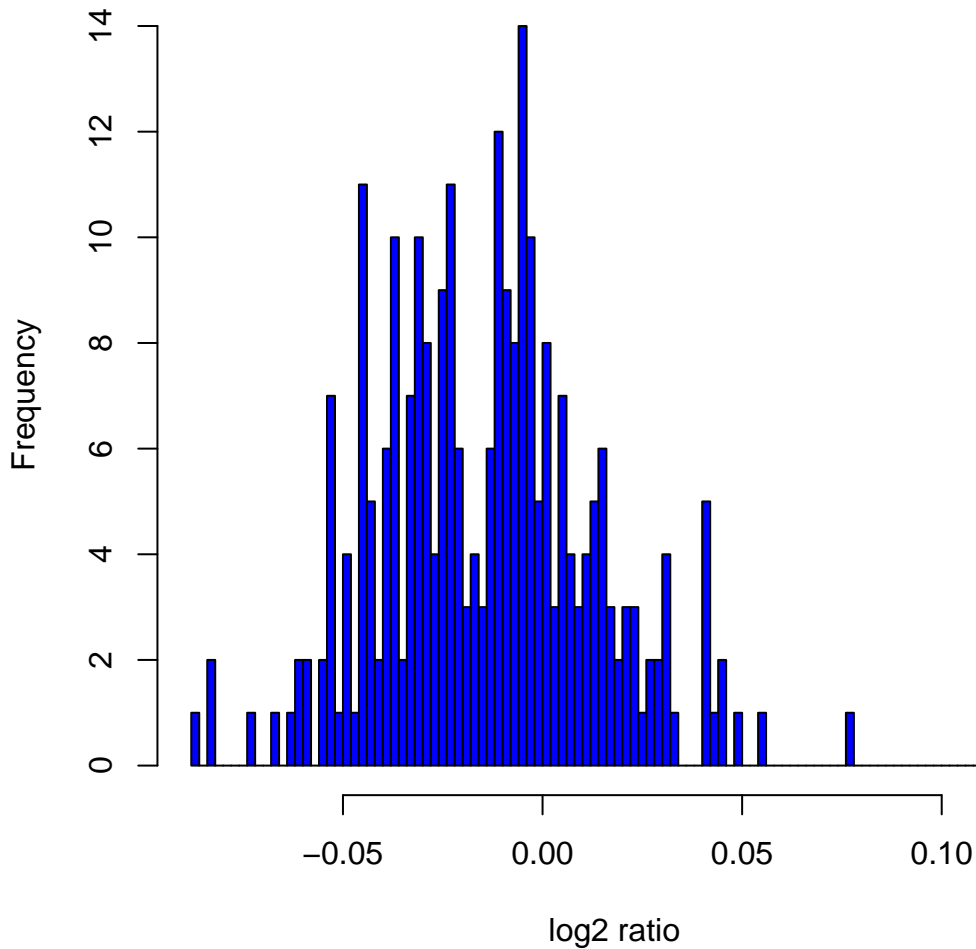
Histogram of \log_2 ratios in 270 HapMap samples at clone Chr5tp-25F9
