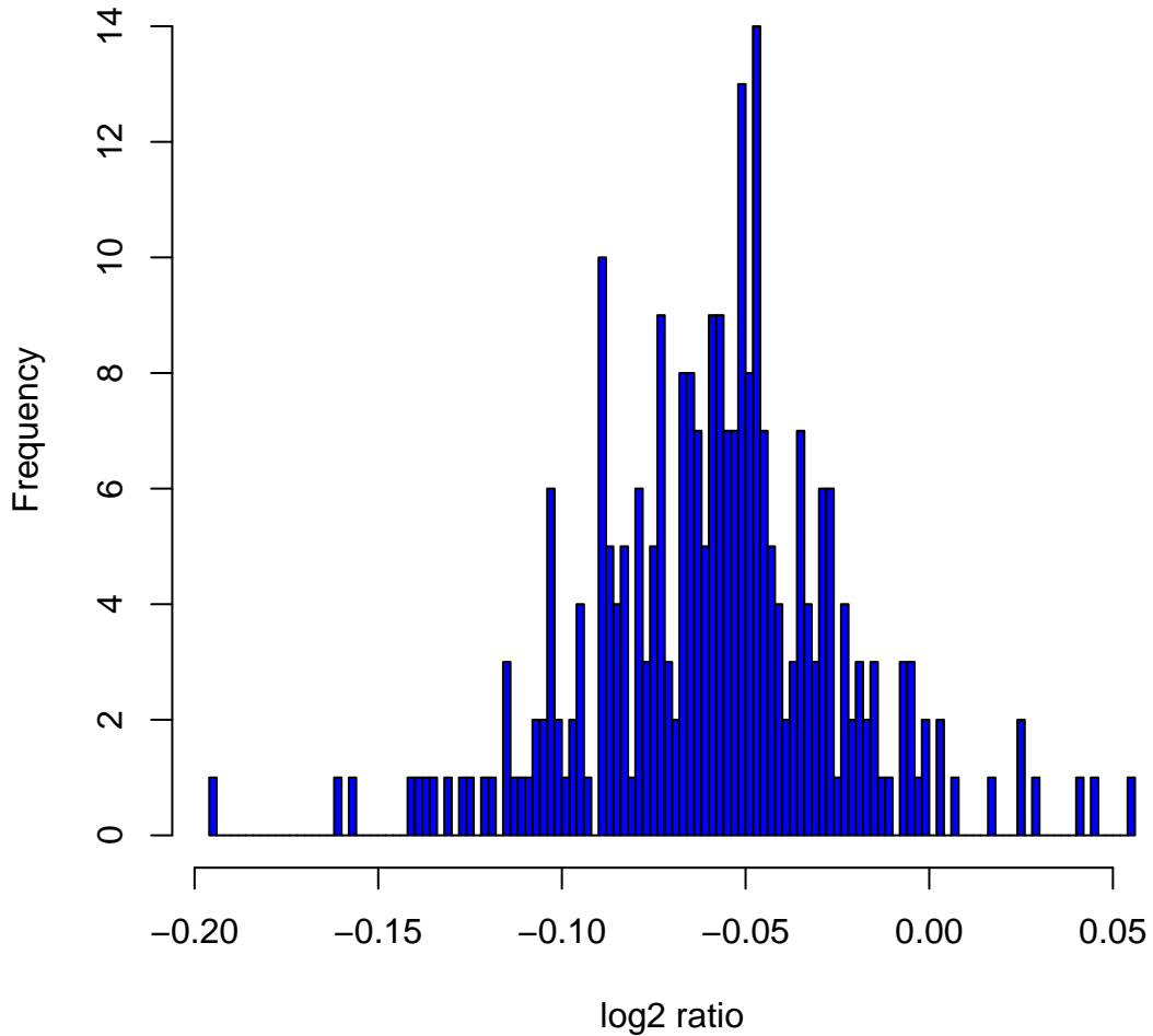
Histogram of \log_2 ratios in 270 HapMap samples at clone Chr5tp-25G4
