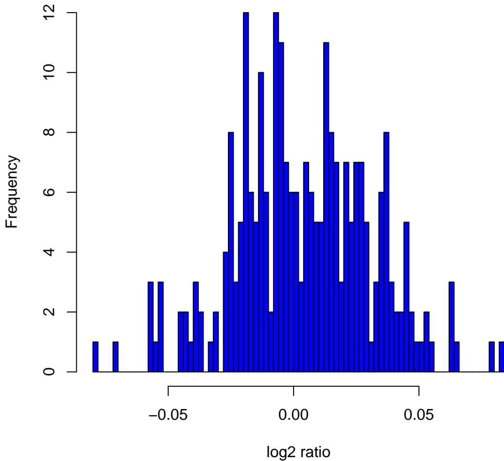
Histogram of log 2 ratios in 270 HapMap samples at clone Chr5tp-25H1
