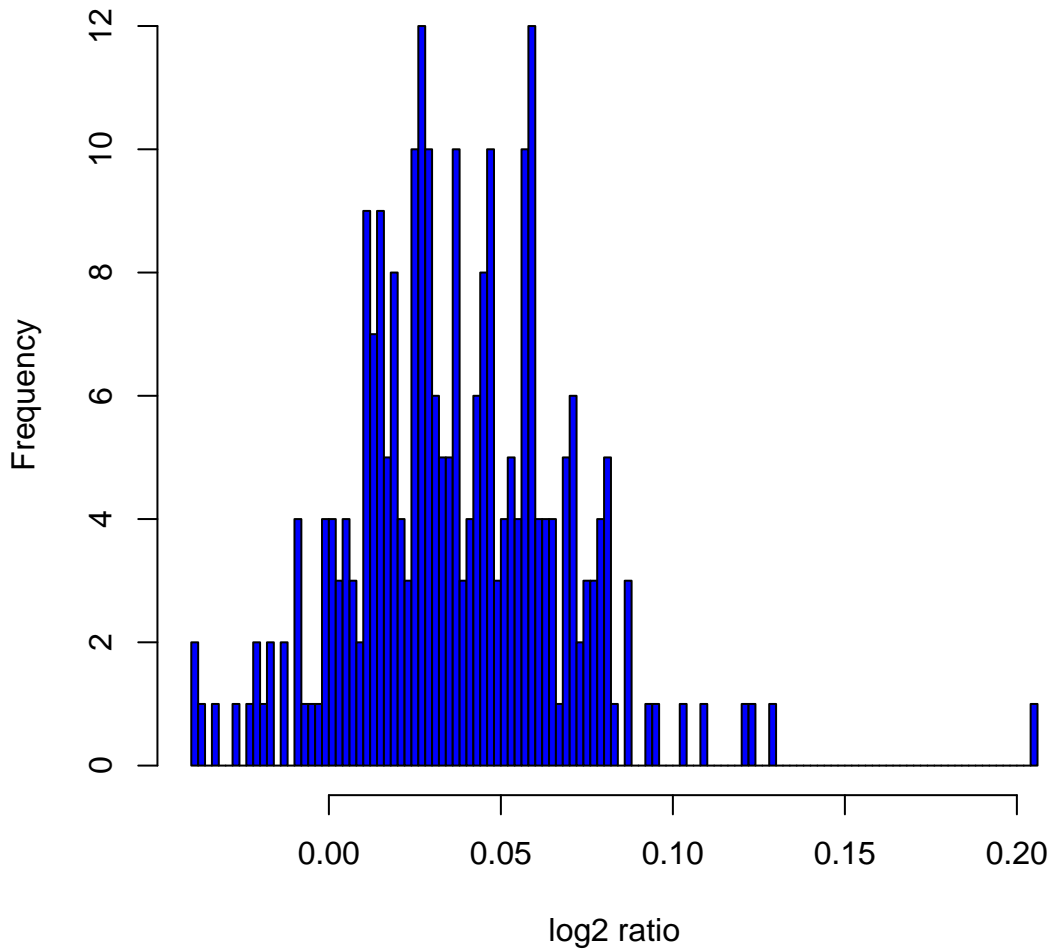
Histogram of log 2 ratios in 270 HapMap samples at clone Chr5tp-2C6
