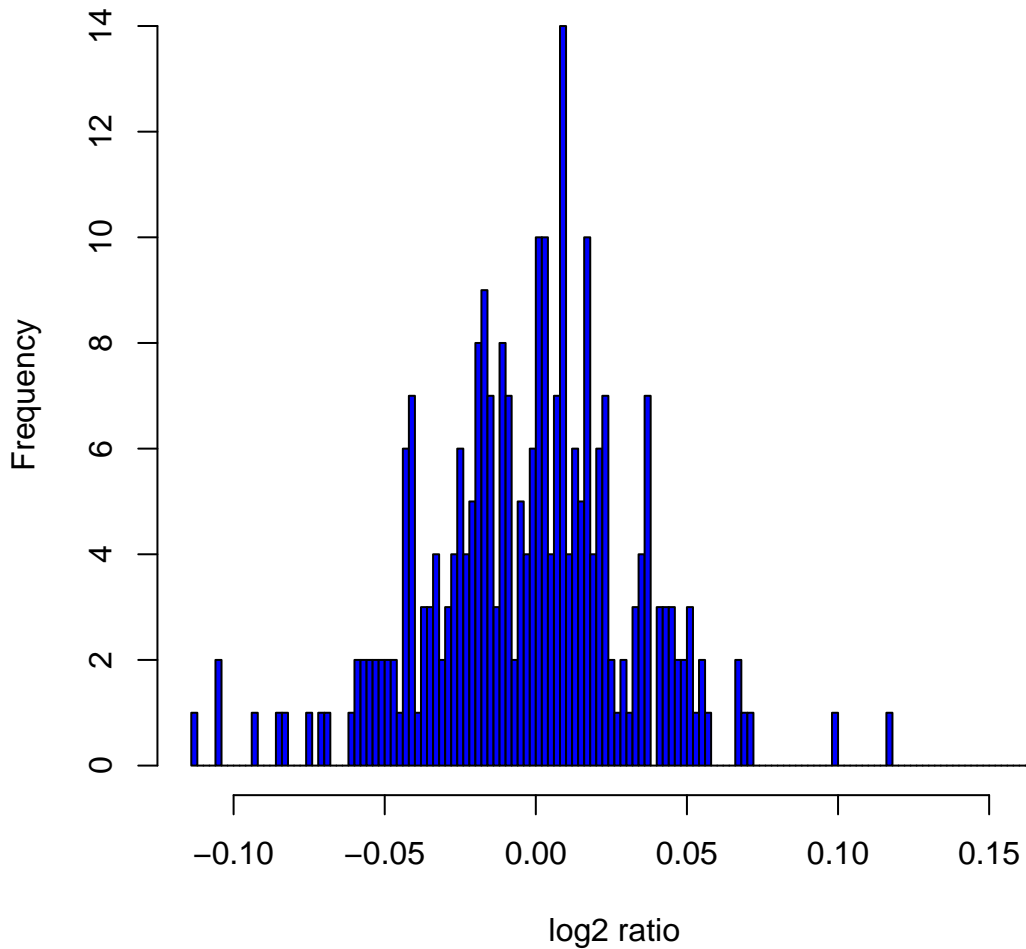
Histogram of log 2 ratios in 270 HapMap samples at clone Chr5tp-2D4
