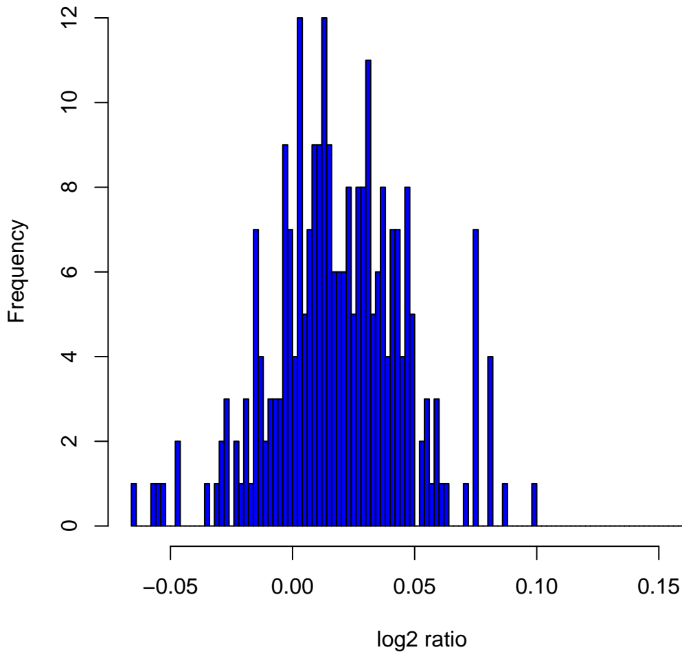
Histogram of log 2 ratios in 270 HapMap samples at clone Chr5tp-2D9
