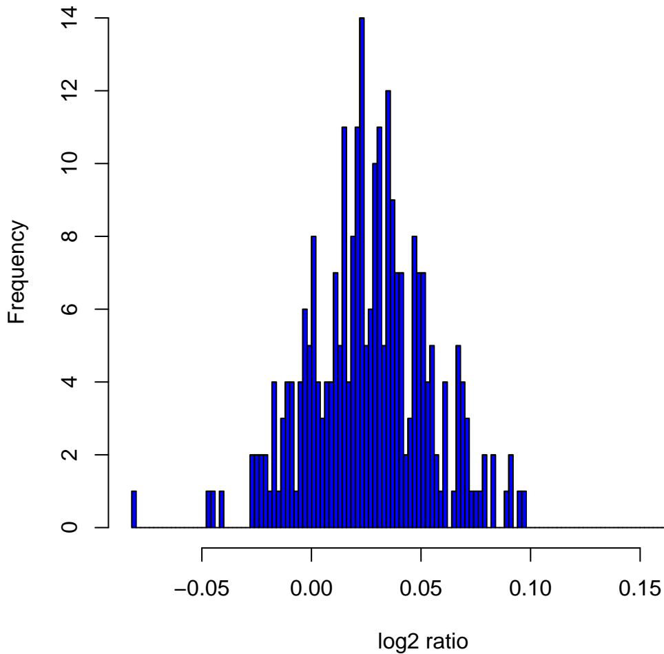
Histogram of log 2 ratios in 270 HapMap samples at clone Chr5tp-2E5
