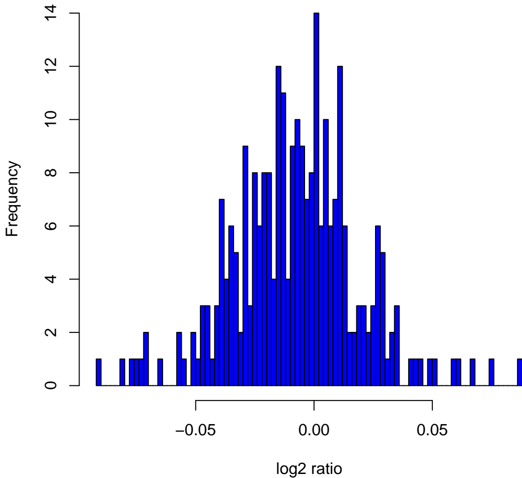
Histogram of log 2 ratios in 270 HapMap samples at clone Chr5tp-2E8
