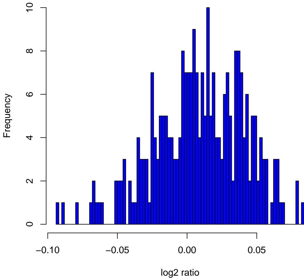
Histogram of log 2 ratios in 270 HapMap samples at clone Chr5tp-2G3
