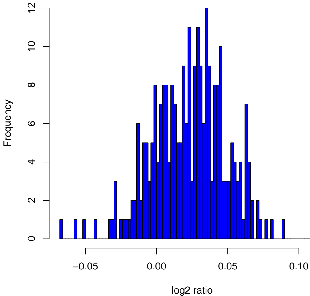
Histogram of log 2 ratios in 270 HapMap samples at clone Chr5tp-3A4
