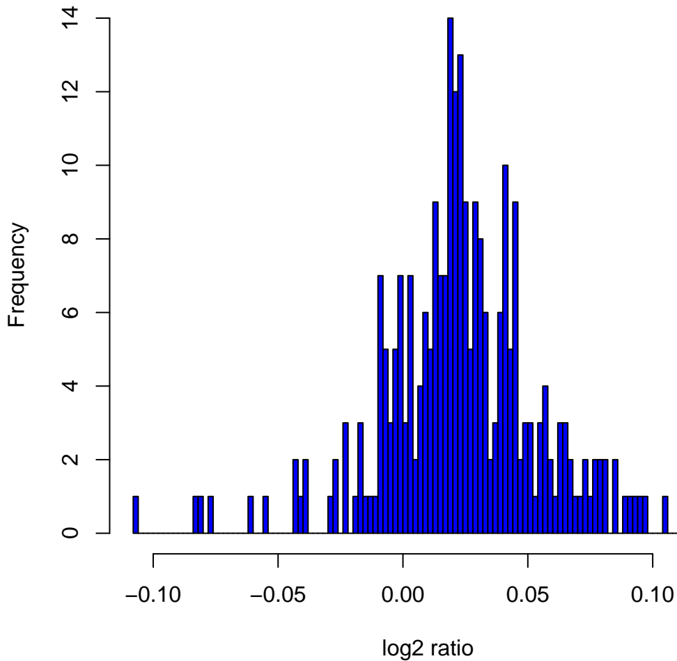
Histogram of log 2 ratios in 270 HapMap samples at clone Chr5tp-3D2
