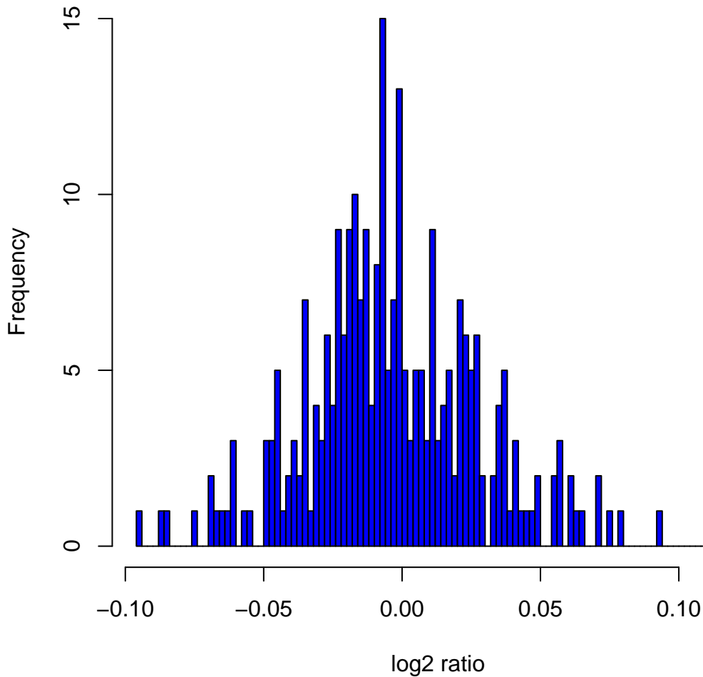
Histogram of log2ratios in 270 HapMap samples at clone Chr5tp-3F3
