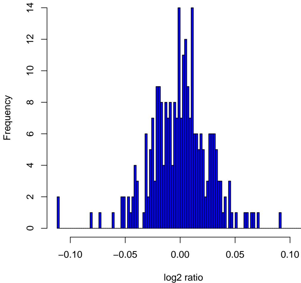
Histogram of log 2 ratios in 270 HapMap samples at clone Chr5tp-3G9
