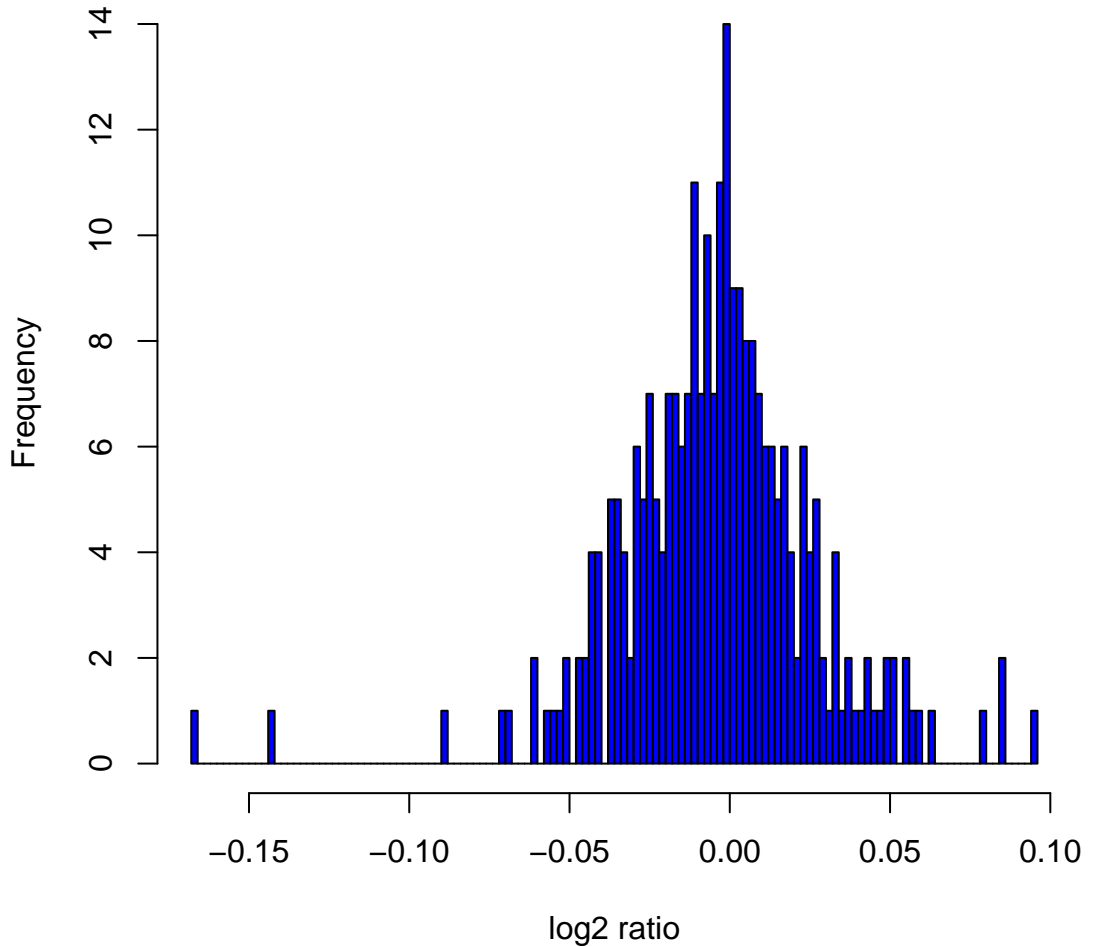
Histogram of log 2 ratios in 270 HapMap samples at clone Chr5tp-4A12
