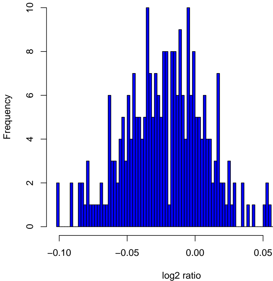
Histogram of \log_2 ratios in 270 HapMap samples at clone Chr5tp-4A5
