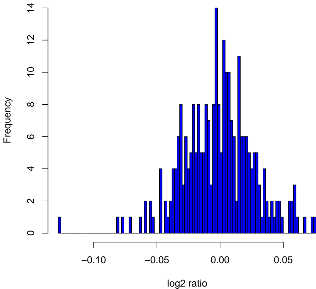
Histogram of log 2 ratios in 270 HapMap samples at clone Chr5tp-4B11
