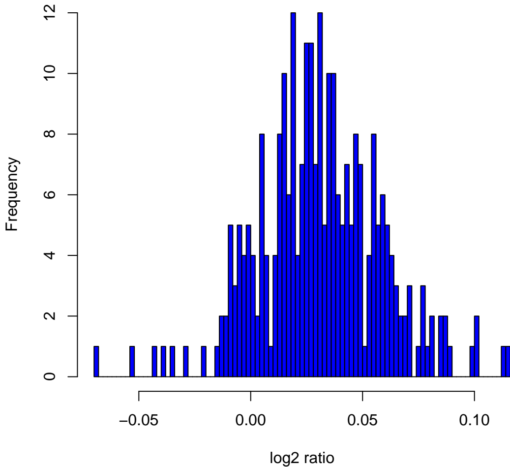
Histogram of log2ratios in 270 HapMap samples at clone Chr5tp-4C6
