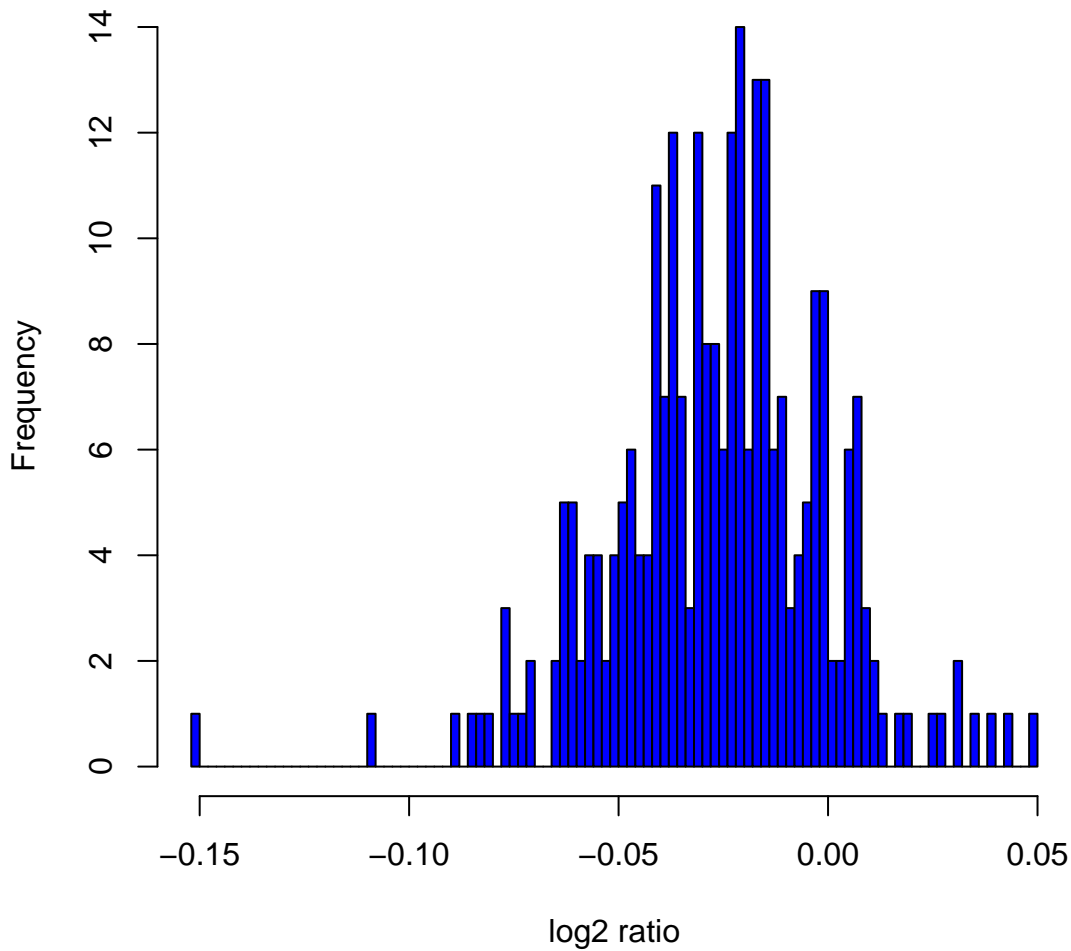
Histogram of log 2 ratios in 270 HapMap samples at clone Chr5tp-4D10
