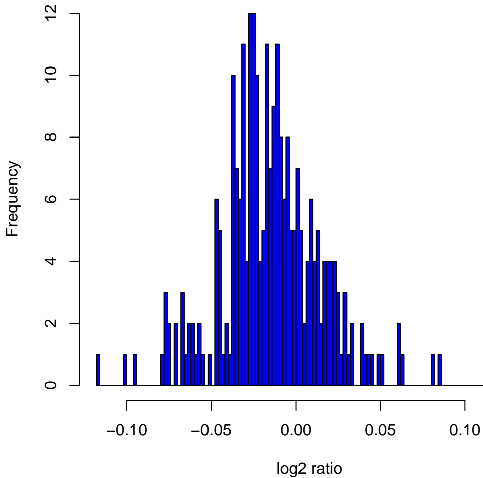
Histogram of log 2 ratios in 270 HapMap samples at clone Chr5tp-4E5
