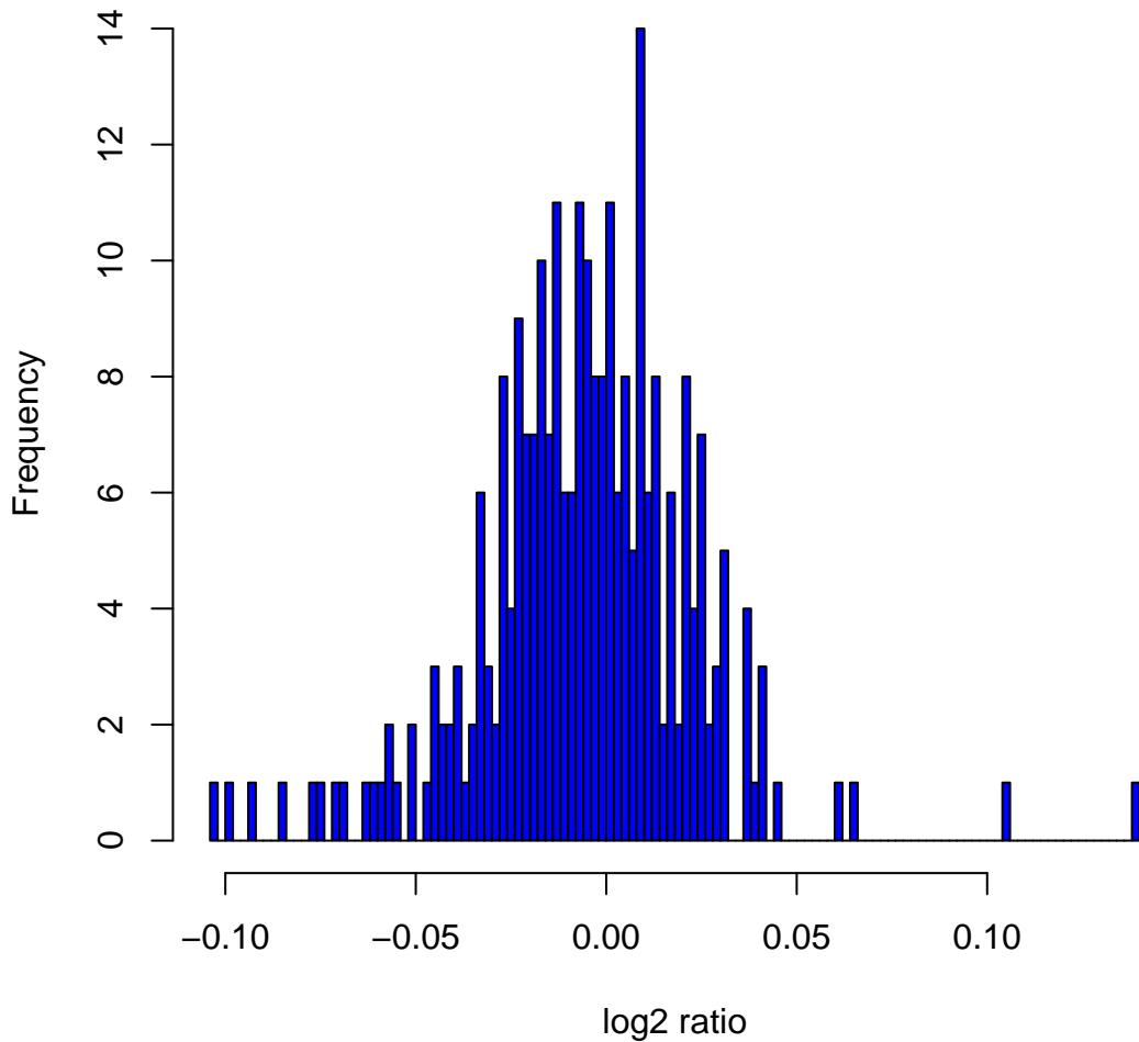
Histogram of log 2 ratios in 270 HapMap samples at clone Chr5tp-4F9
