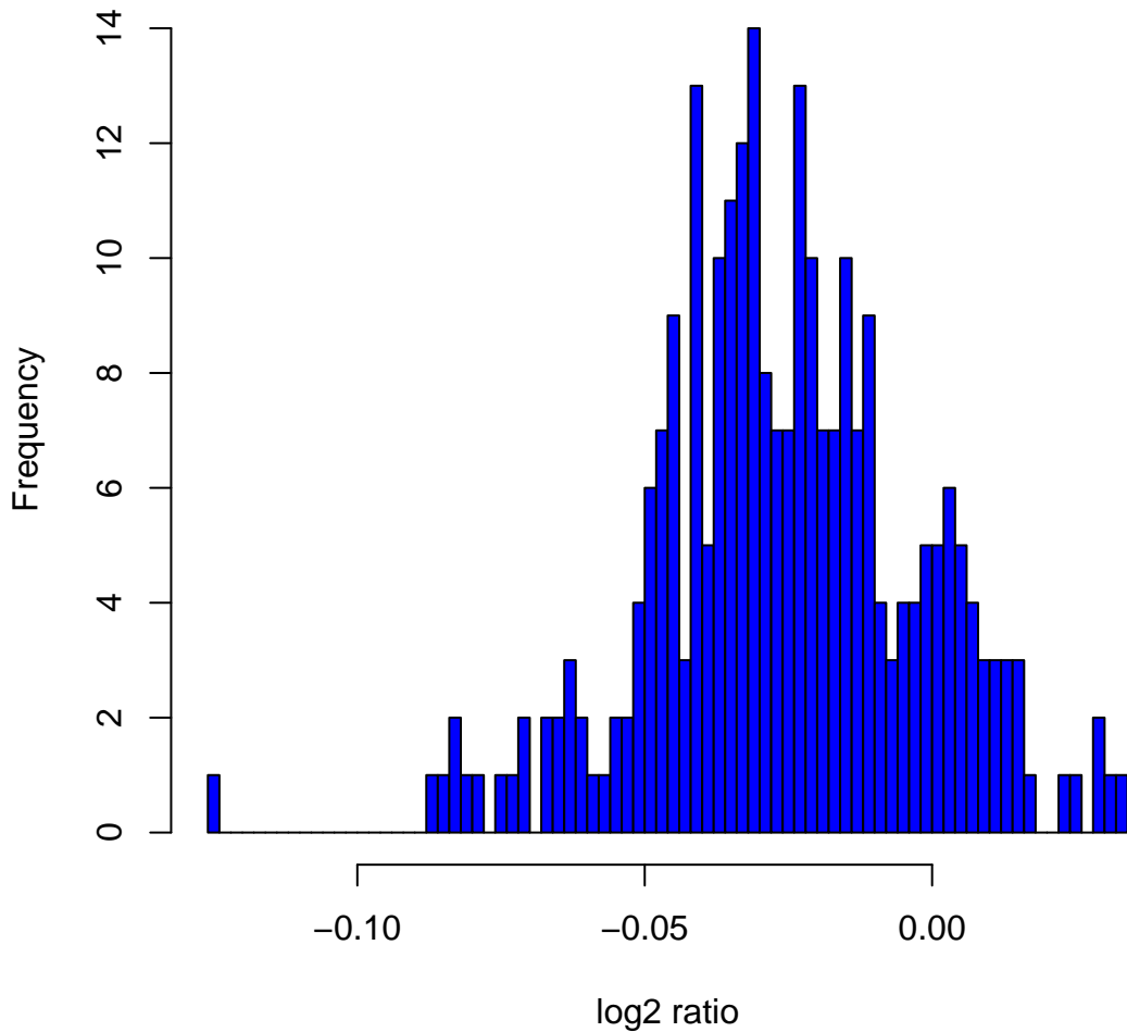
Histogram of log 2 ratios in 270 HapMap samples at clone Chr5tp-4H1
