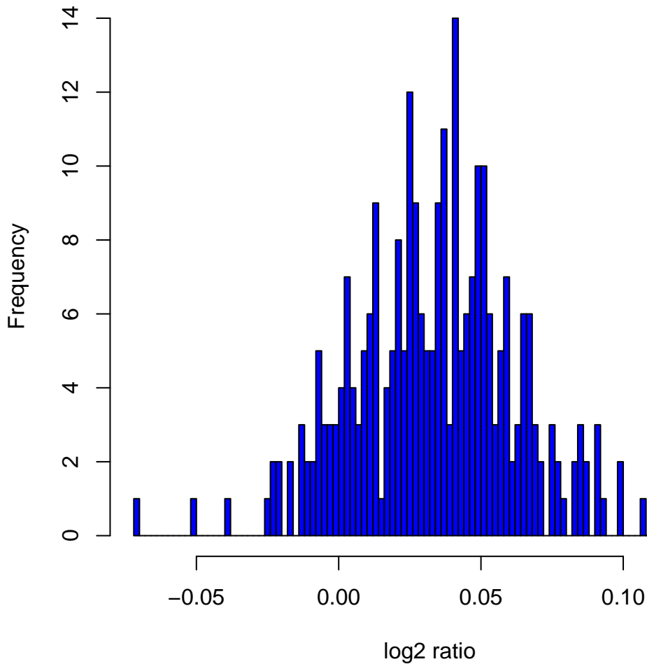
Histogram of log 2 ratios in 270 HapMap samples at clone Chr5tp-4H2
