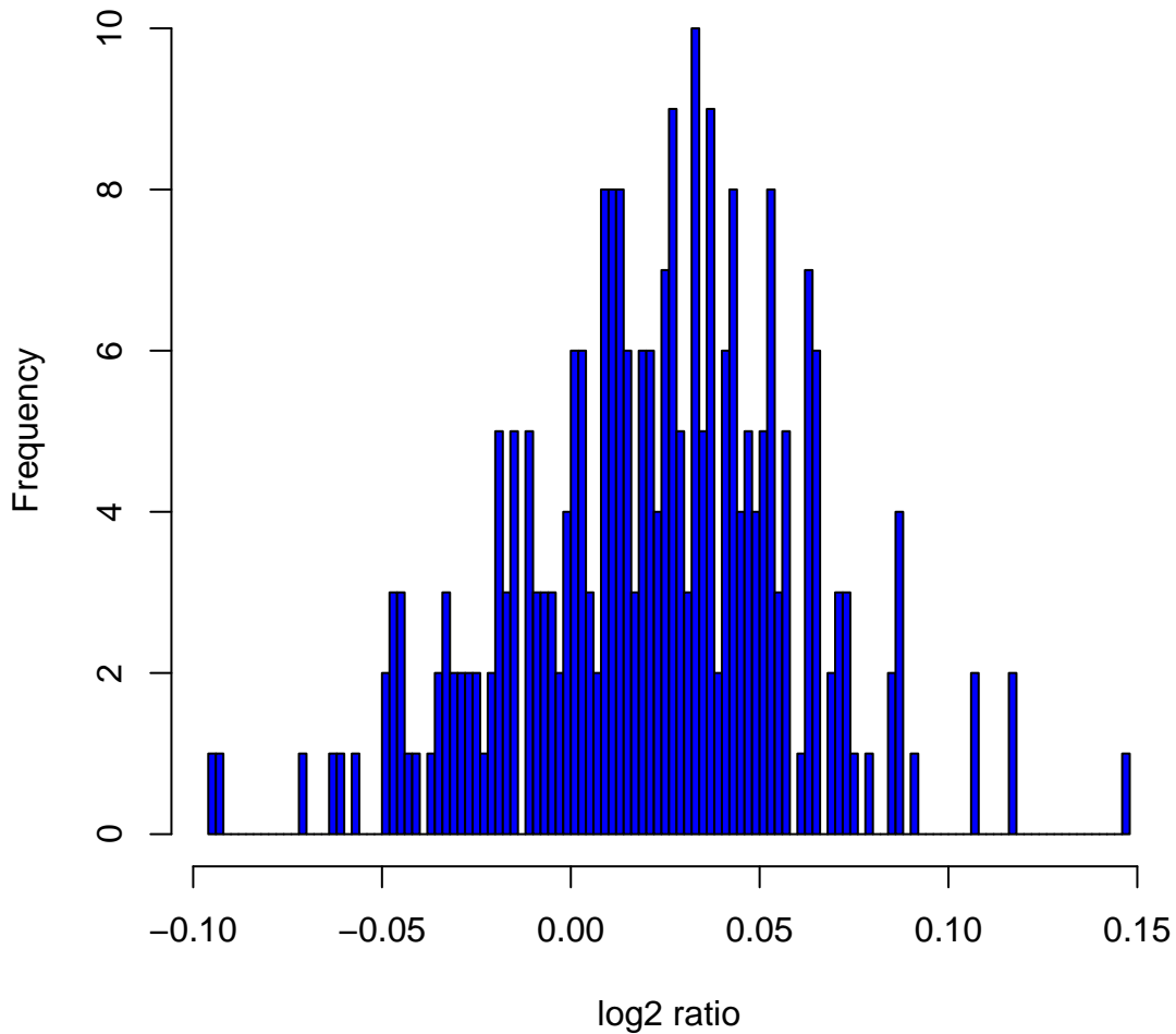
Histogram of log 2 ratios in 270 HapMap samples at clone Chr5tp-4H3
