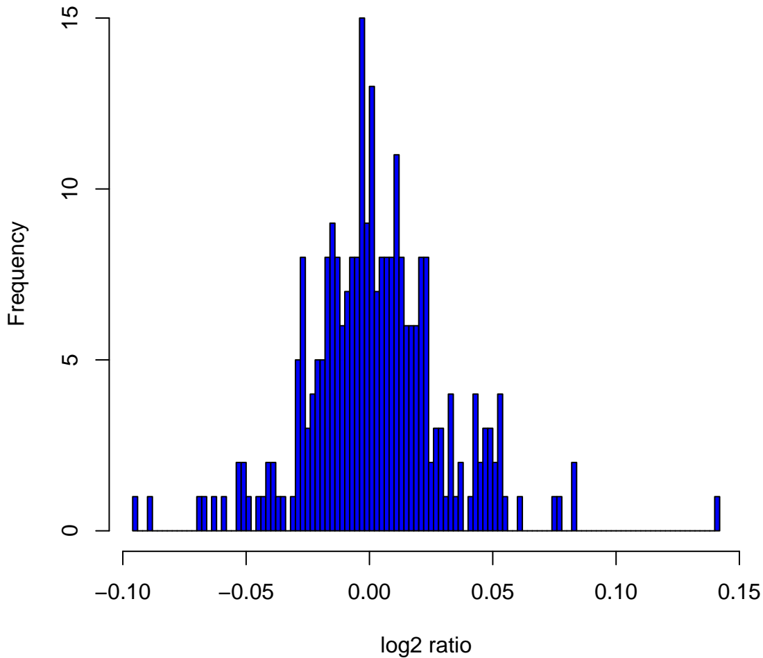
Histogram of log 2 ratios in 270 HapMap samples at clone Chr5tp-5A1
