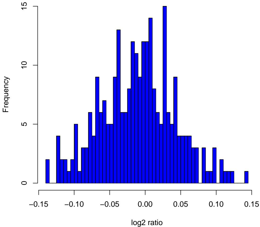
Histogram of log 2 ratios in 270 HapMap samples at clone Chr5tp-5A11
