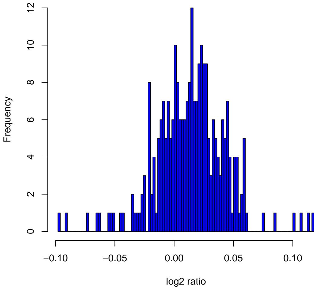
Histogram of \log_2 ratios in 270 HapMap samples at clone Chr5tp-5A7
