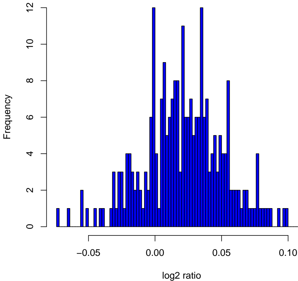
Histogram of log 2 ratios in 270 HapMap samples at clone Chr5tp-5B1
